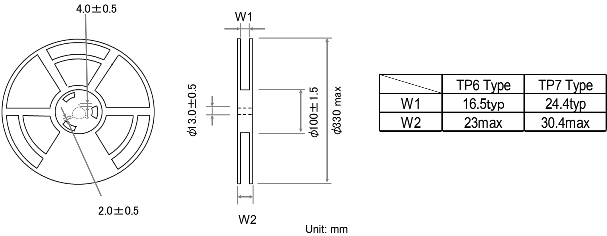
Figure 4 Reel Forms
