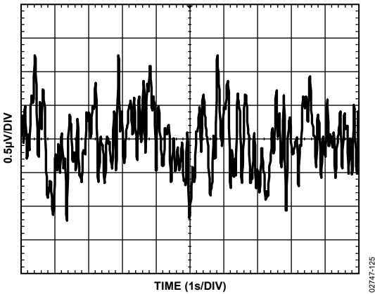
Figure 25. ADR02 Typical Noise Voltage, 0.1 Hz to 10.0 Hz
