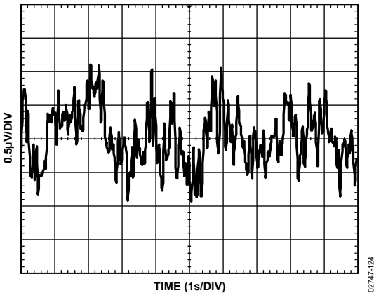
Figure 24. ADR01 Typical Noise Voltage, 0.1 Hz to 10.0 Hz
