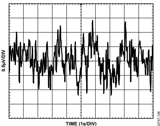
Figure 26. ADR03 Typical Noise Voltage, 0.1 Hz to 10.0 Hz
