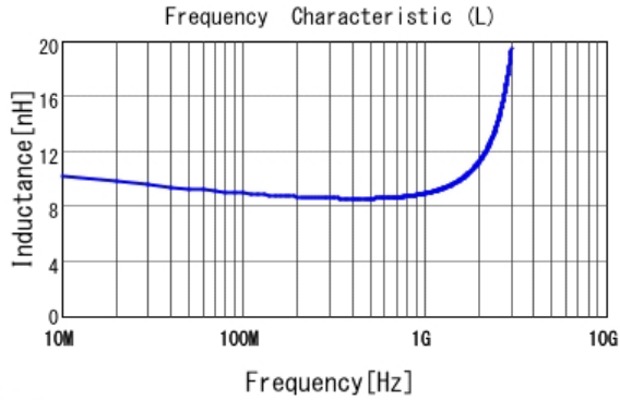
■ LQG15HS9N1J02 L
