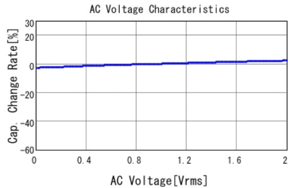
■ GRM033R71C101KA01 C-AC Voltage capchange, DCOV, 25.0d
