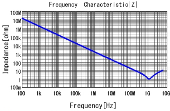
■ GRM033R71C101KA01 |Z| DCOV, 25degC
