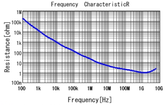
■ GRM033R71C101KA01 R DCOV, 25degC
