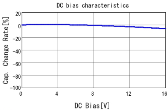
■ GRM033R71C101KA01 C-DC bias capchange, 25.0degC, AC1.
