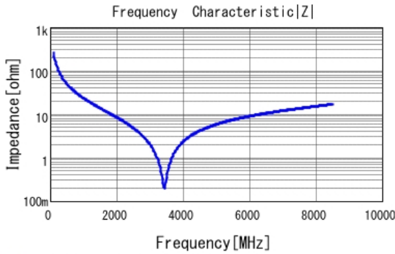
GJM1555C1H6R2BB01 |Z| DC0V, 25degC
