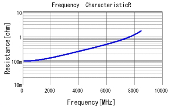
GJM1555C1H6R2BB01 R DC0V, 25degC
