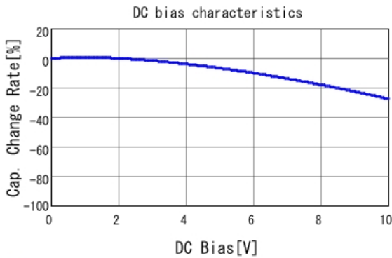
■ GRM033R71A472KA01 C-DC bias capchange, 25.0degC, AC1.
