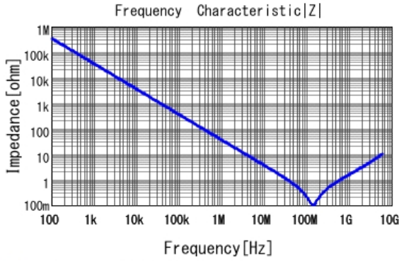
■ GRM033R71A472KA01 |Z| DCOV, 25degC
