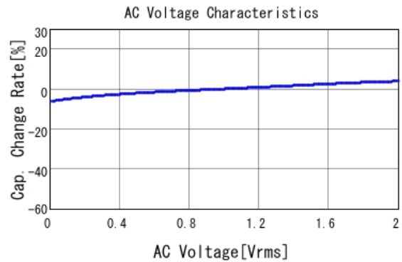
■ GRM033R71A472KA01 C-AC Voltage capchange, DCOV, 25.0d
