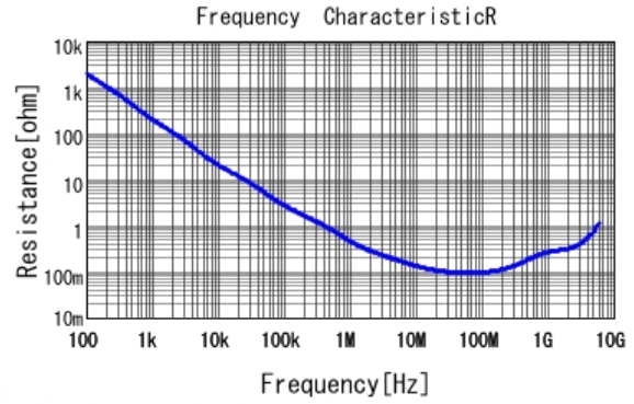
■ GRM033R71A472KA01 R DCOV, 25degC
