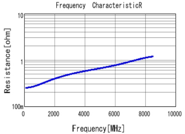
■ GRM0335C1H3R0BA01 R DC0V, 25degC
