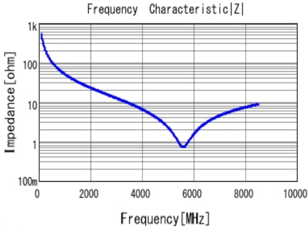
■ GRM0335C1H3R0BA01 |Z| DC0V, 25degC
