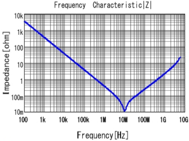
■ GRM188R71A474KA61 |Z| DCOV, 25degC
