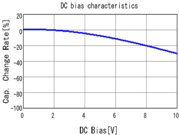
■ GRM188R71A474KA61 C-DC bias capchange, 25.0degC, AC1.
