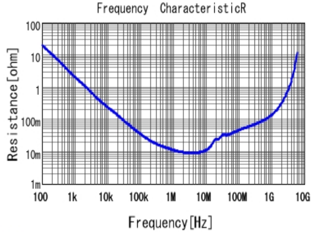
■ GRM188R71A474KA61 R DCOV, 25degC
