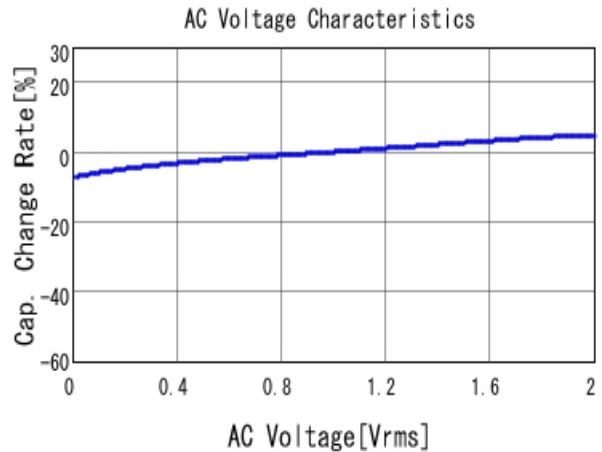
■ GRM188R71A474KA61 C-AC Voltage capchange, DCOV, 25.0d
