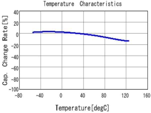
■ GRM188R71A474KA61 C-Temp. capchange, DC0.0V, AC1.0V r m
