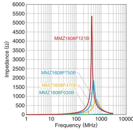
MMZ1608F series
