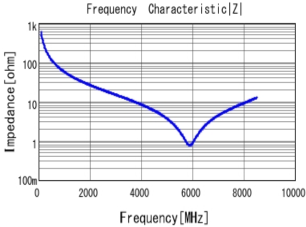
■ GRM0335C1H2R7CA01 |Z| DC0V, 25degC
