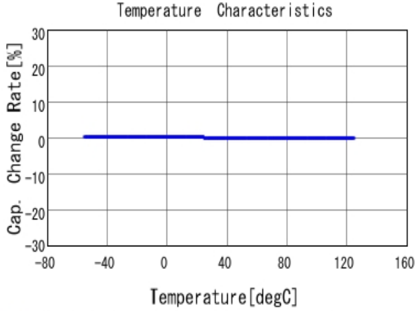
■ GRM0335C1H2R7CA01 C-Temp. capchange, DCOV, AC1Vrms
