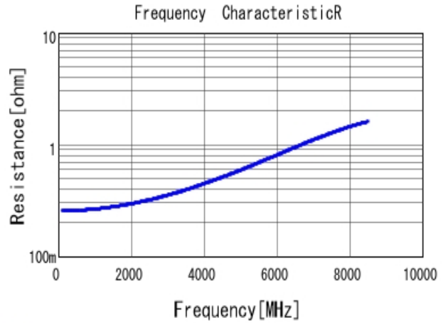
■ GRM0335C1H2R7CA01 R DC0V, 25degC
