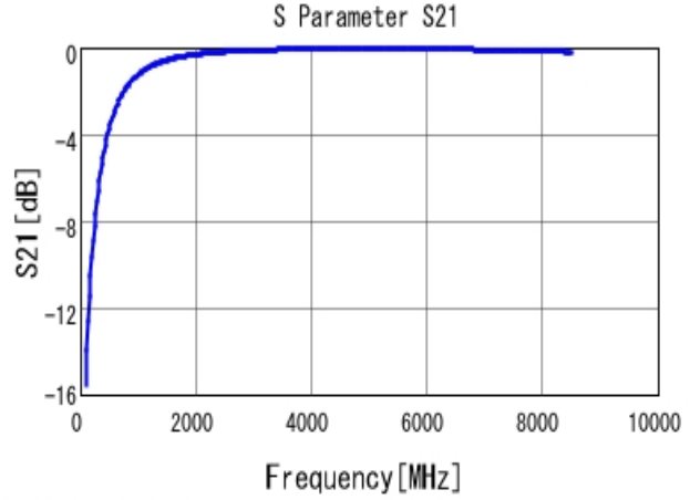
■ GRM0335C1H2R7CA01 S21 DCOV, 25degC
