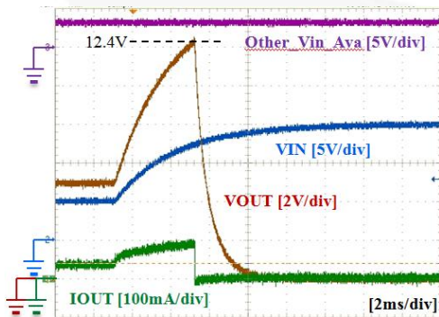
Figure 29. V_{IN} Over-Voltage Protection Response ( V_{IN}=5 V \rightarrow 15 V, V_{BUS}=5 V, EN=V_{IN\_SEL}=HIGH , C_{OUT}=4.7 \mu F , R_L=150 \Omega )
