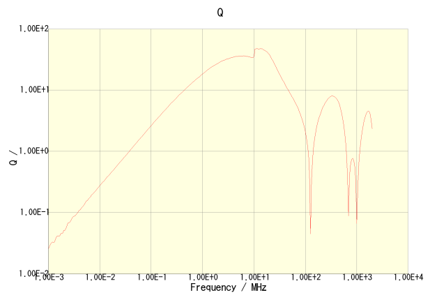
NLV32T-2R2J-PF
