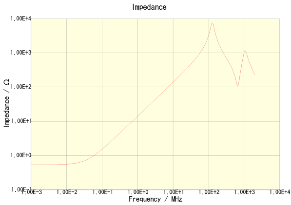
NLV32T-2R2J-PF
