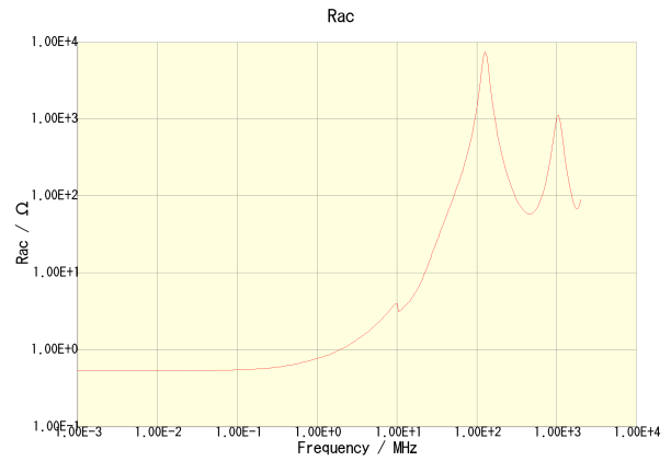
NLV32T-2R2J-PF
