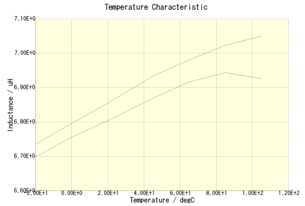
NLCV32T-6R8M-EF(DC = 0A)
