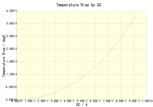
NLCV32T-6R8M-EF(Amb. Temp. = 20degc)
