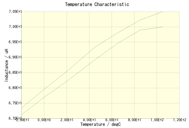
NLCV32T-680K-PF(DC = 0A)
