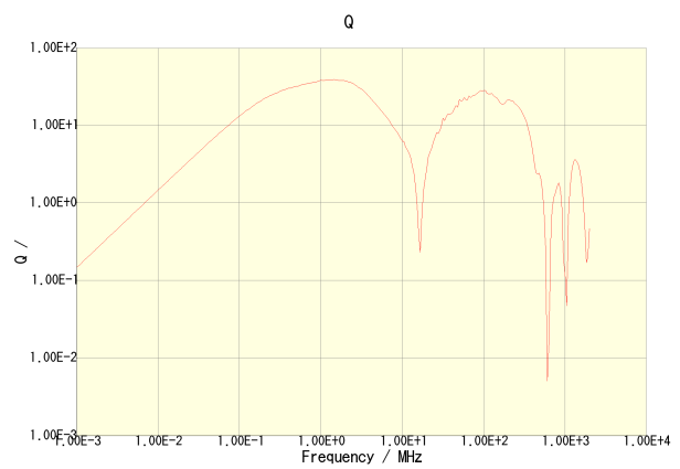
NLCV32T-680K-PF
