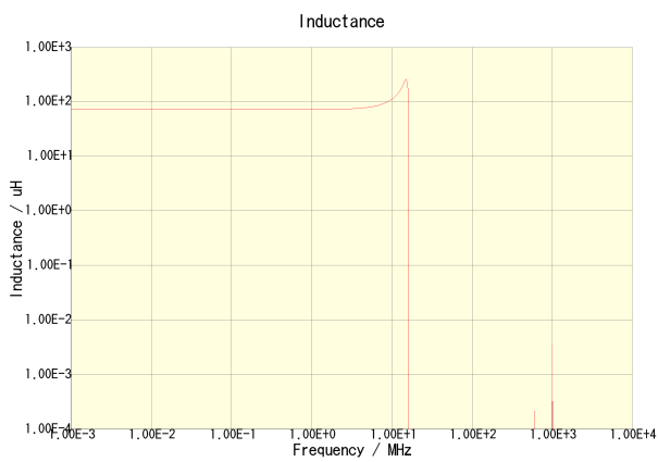
NLCV32T-680K-PF
