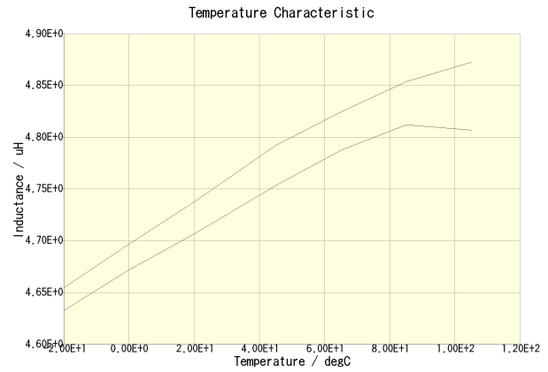
NLCV32T-4R7M-EF(DC = 0A)
