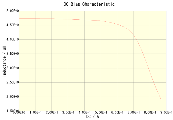
NLCV32T-4R7M-EF(Amb. Temp. = 20degC)
