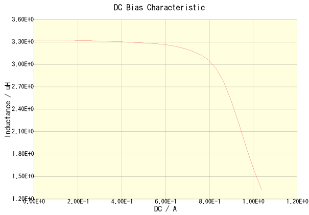
NLCV32T-3R3M-EF(Amb. Temp. = 20degc)
