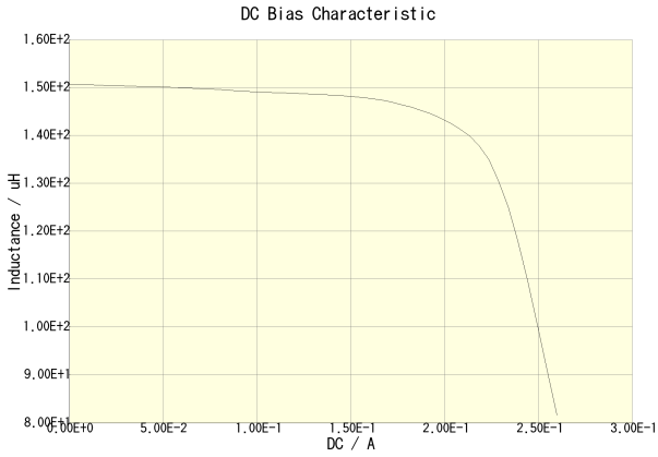
NLC453232T-151K-PF(Amb. Temp. = 20degc)
