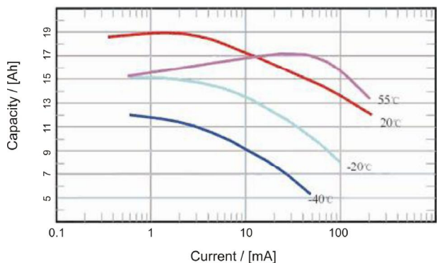
Temperature characteristics
