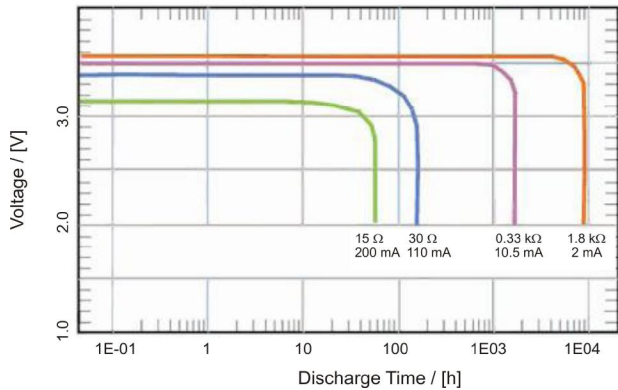
Continuous Discharges at 25 °C (77 °F)
