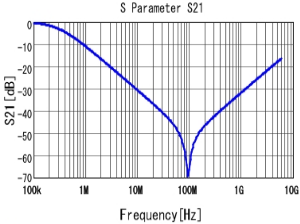
■ NFM41CC223R2A3 S21 DC0V, 25degC, Feedthrough
