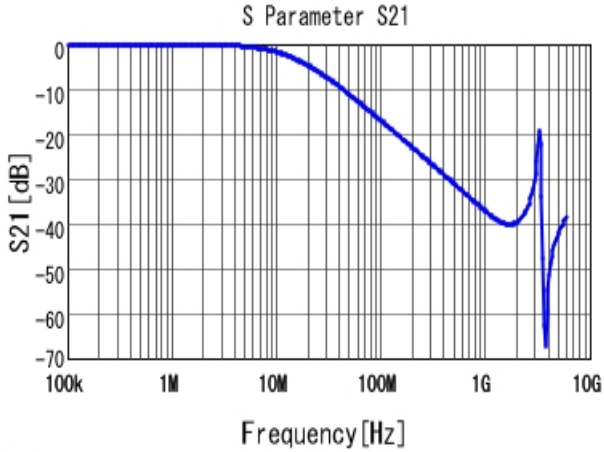
■ NFM3DCC471R1H3 S21 DC0V, 25degC, Feedthrough
