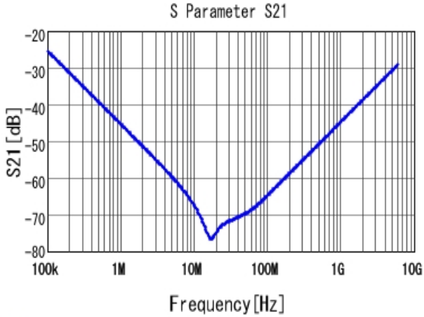
■ NFM18PC225B0J3 S21 DC0V, 25degC, Feedthrough
