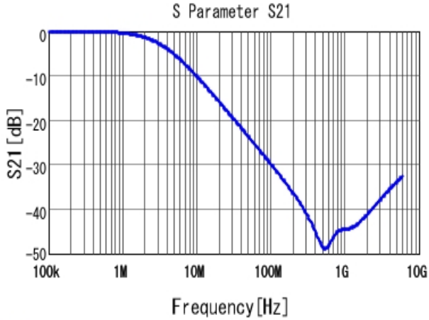
■ NFM18CC222R1C3 S21 DCOV, 25degC, Feedthrough
