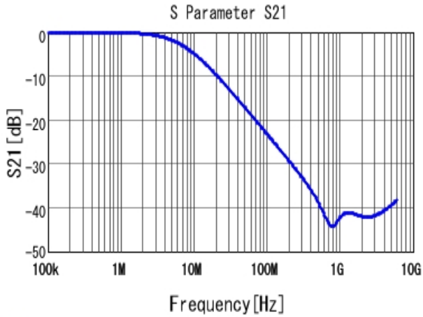
■ NFM18CC102R1C3 S21 DCOV, 25degC, Feedthrough
