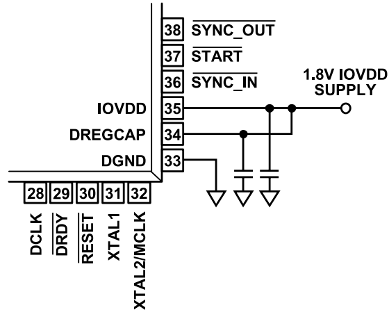
Figure 75. DREGCAP and IOVDD Connection Diagram for 1.8 V IOVDD Operation
