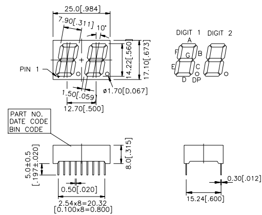
B. LTD-5X21A/5X23A
