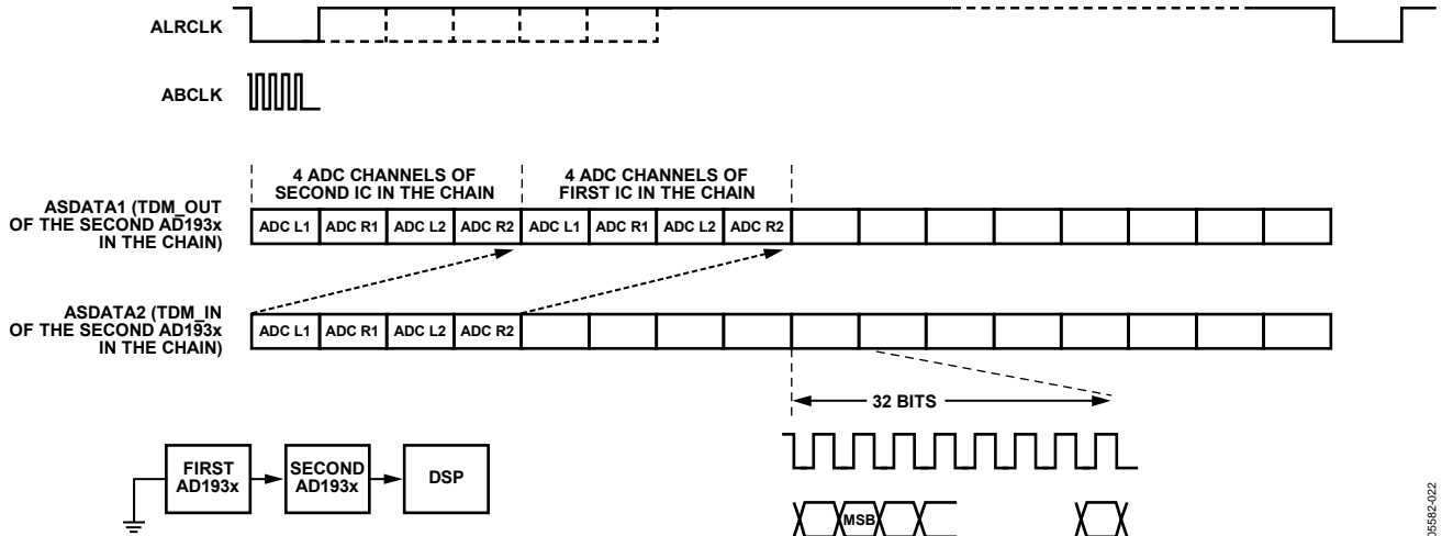
Figure 22. ADC TDM Daisy-Chain Mode (512 f_s BCLK, Two-AD1938x Daisy Chain)
