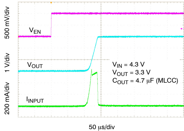
Figure 33. Enable Turn-on Response – C_{OUT} = 4.7\ \mu\text{F} , I_{OUT} = 10\ \text{mA}
