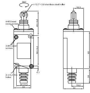
Direction of rotor CHL-5220
