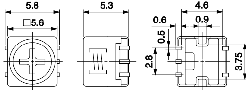
(Unit: mm)
