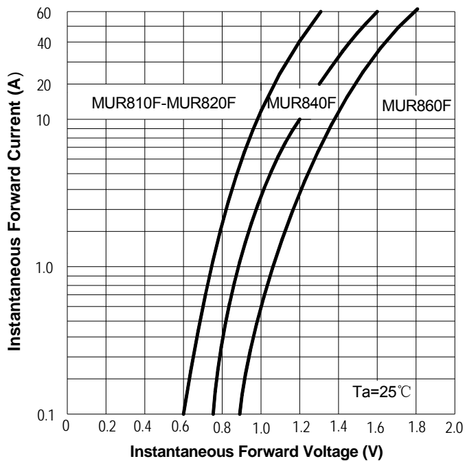
FIG3: Forward Voltage
