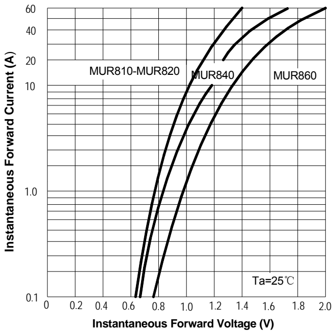
FIG3: Forward Voltage
