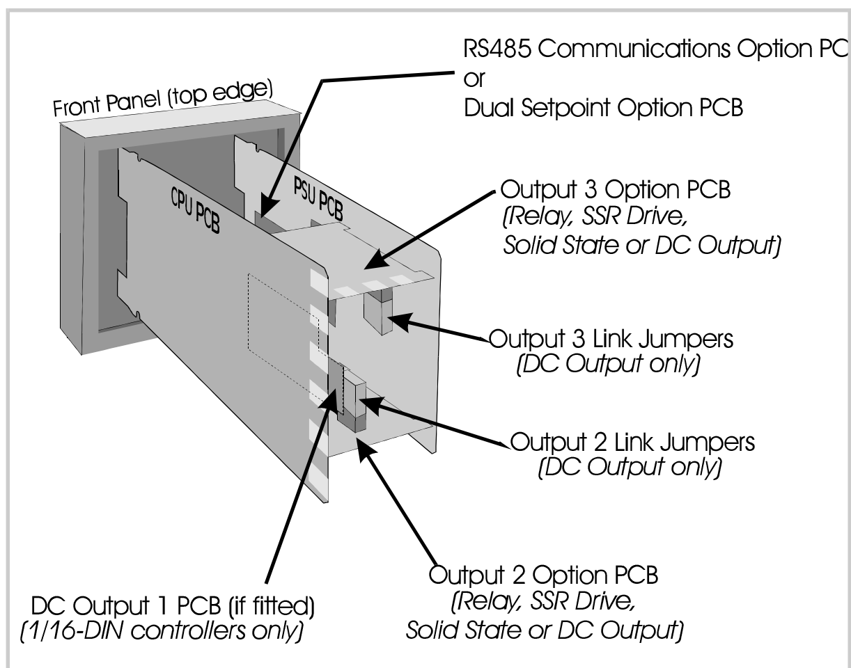
Figure 2-1 PCB Positions
