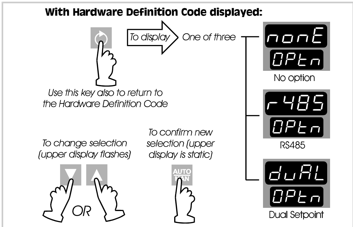
Figure 3-3 Option Selection
