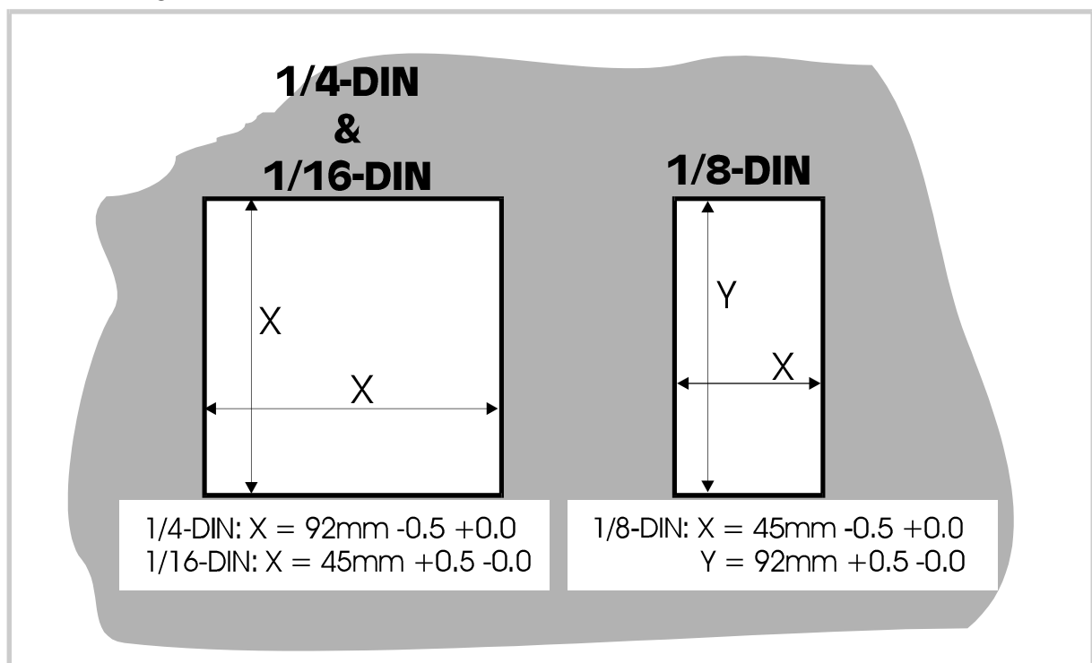
Figure 1-1 Cut-out Dimensions
