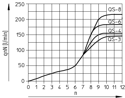
Standard nominal flow rate q_{nN} at 6 \rightarrow 5 bar as a function of turns of the adjusting screw n GRLA/GRLZ-1/8
