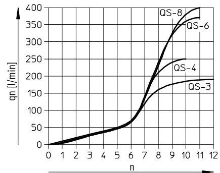
Standard flow rate q_n at 6 \rightarrow 0 bar as a function of turns of the adjusting screw n GRLA/GRLZ-1/8
