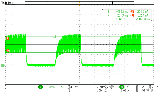
90Vac CH4: Io
