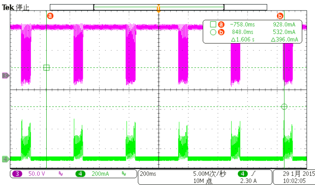
90Vac CH3:Vds CH4:IL
