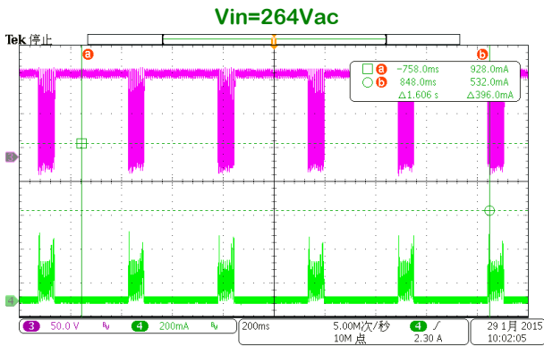
264Vac CH3:Vds CH4:Ic
