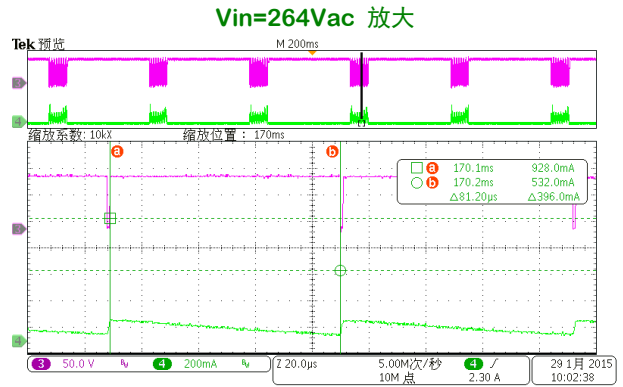
264Vac CH3:Vds CH4:Ic
