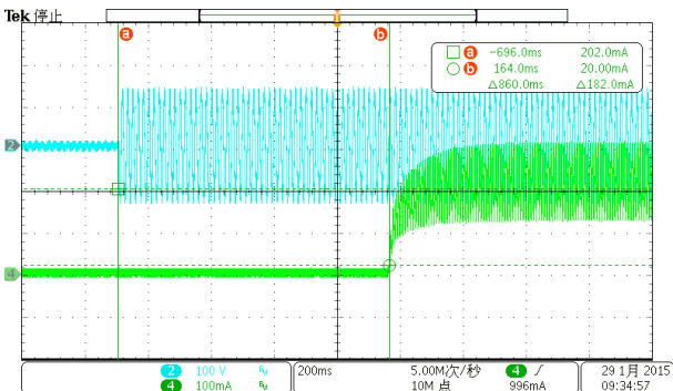
90Vac CH3: Vin-ac CH4: Io
