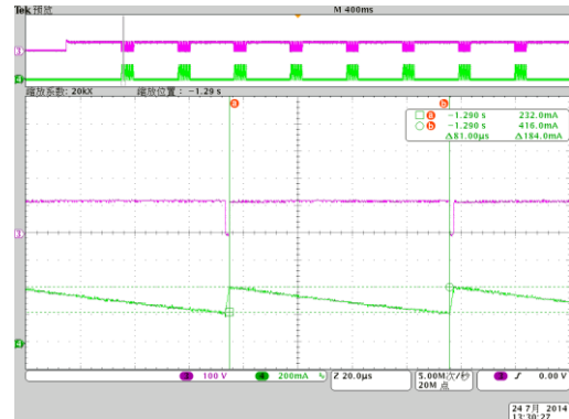
90Vac CH3:Vds CH4:IL
