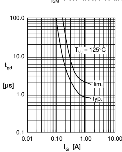
Fig. 5 Gate controlled delay time t_{gd}
