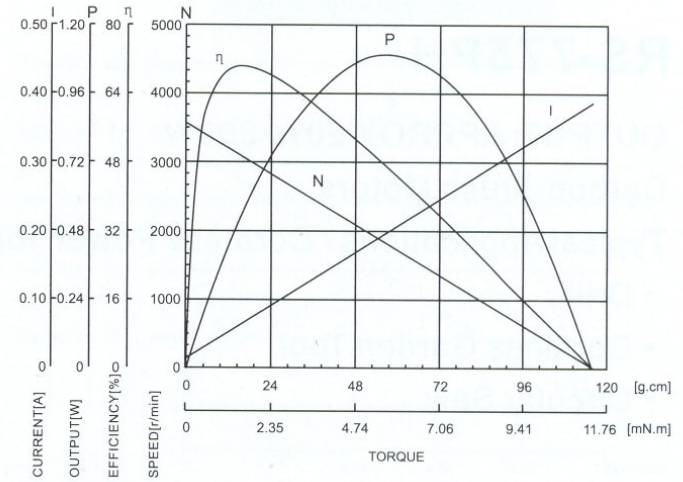
FBGM2431-10520 12.0V
