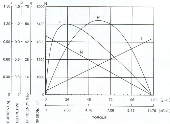
FBGM2431-17180 6.0V
