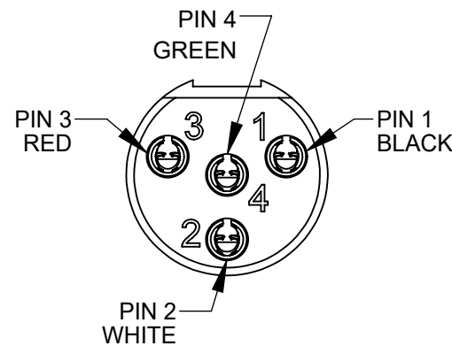
ST-604 FRONT MATING VIEW
