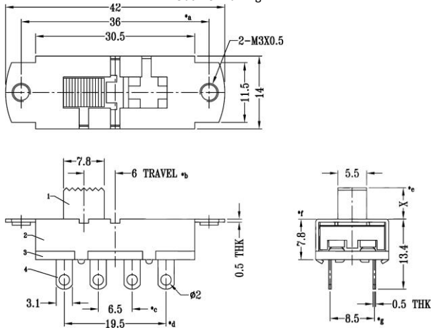
Mounting
