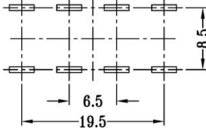
Mounting
