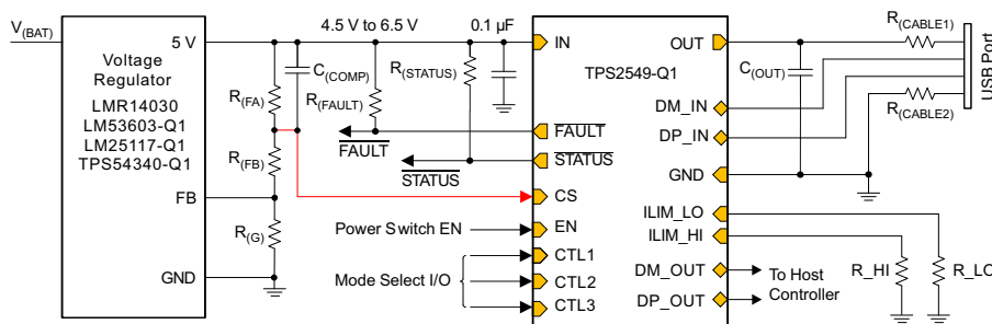
Simplified Schematic
