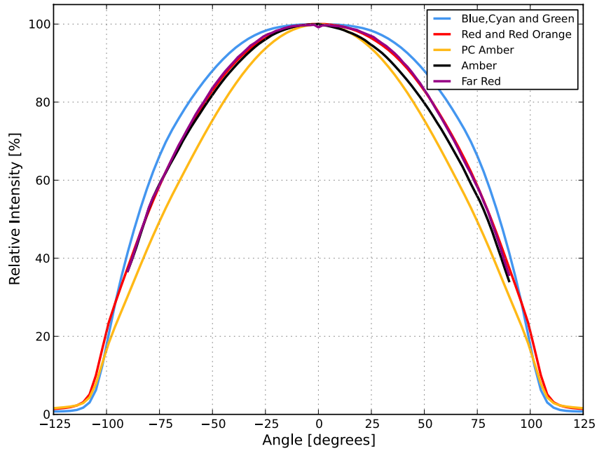
Figure 5a: Typical radiation pattern for LUXEON C Far Red, Red, Red-Orange, PC Amber, Green, Cyan and Blue at 350mA, T_j=85^{\circ}\text{C} .
