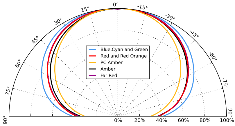
Figure 6a: Typical polar radiation pattern for LUXEON C Far Red, Red, Red-Orange, PC Amber, Green, Cyan and Blue at 350mA, T_j=85^\circ\text{C} .
