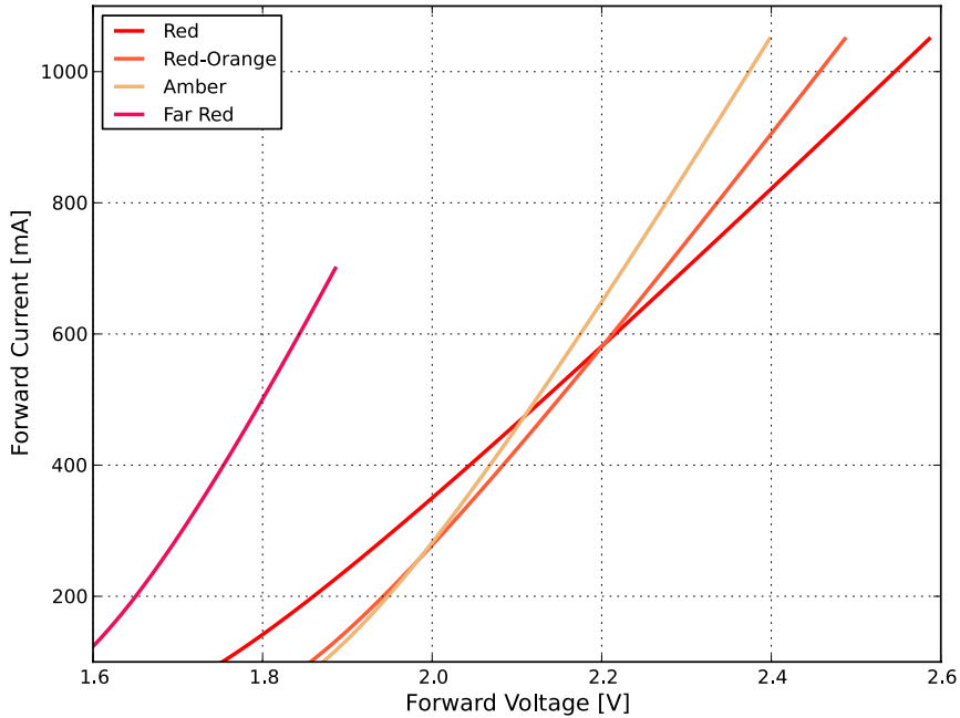
Figure 4a: Typical forward current vs. forward voltage for LUXEON C Red and Red-Orange at T_j=85^\circ\text{C} .
