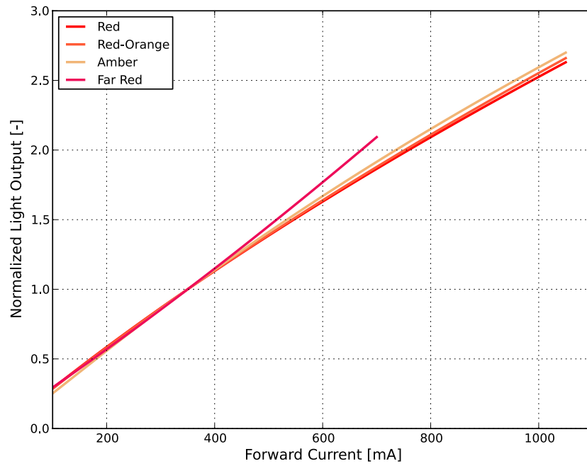
Figure 3a: Typical normalized light output vs. forward current for LUXEON C Far Red, Red, Red-Orange and Amber at T_j=85^\circ\text{C} .
