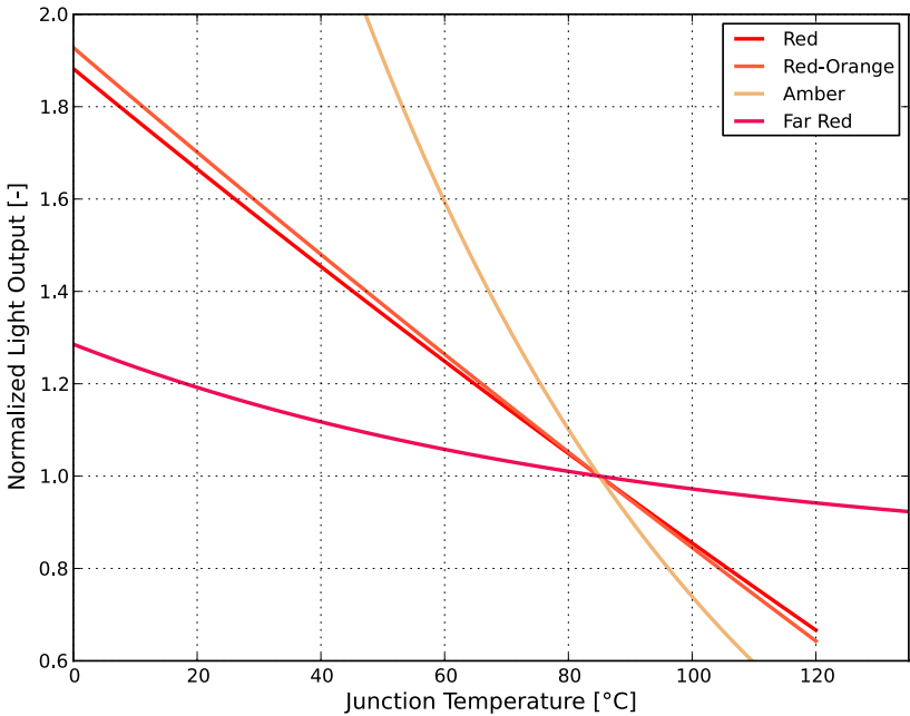
Figure 2a: Typical normalized light output vs. junction temperature for LUXEON C Far Red, Red, Red-Orange and Amber at 350mA.
