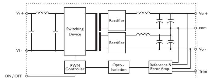
• Block diagram for FDD25 series with dual output
