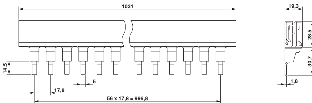
Dimensional drawing
