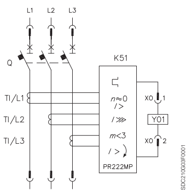
Three-pole circuit-breaker with PR222MP electronic trip unit
