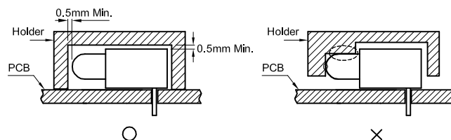
" ○ " Correct mounting method " x " Incorrect mounting method
