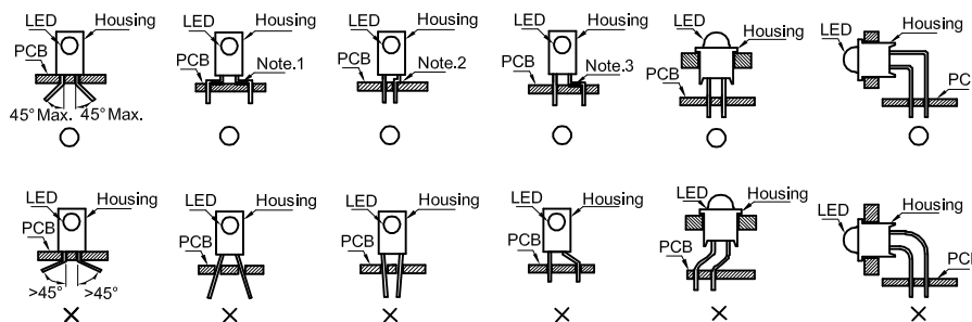
" ○ " Correct mounting method " x " Incorrect mounting method
