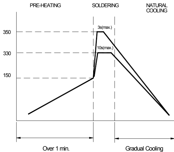
Figure 2. Hand Soldering
