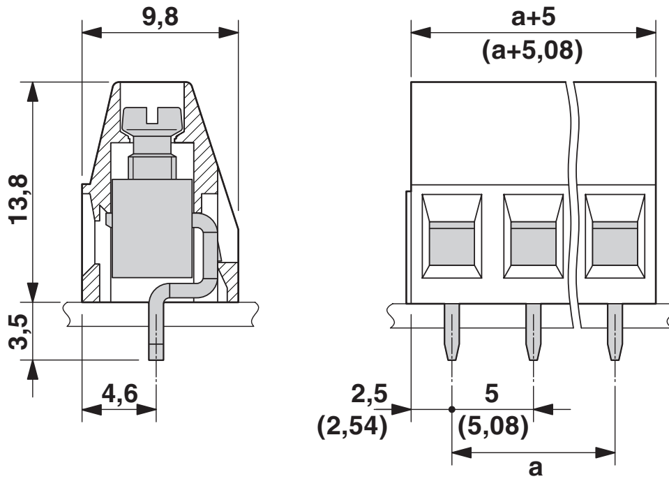
Dimensional drawing
