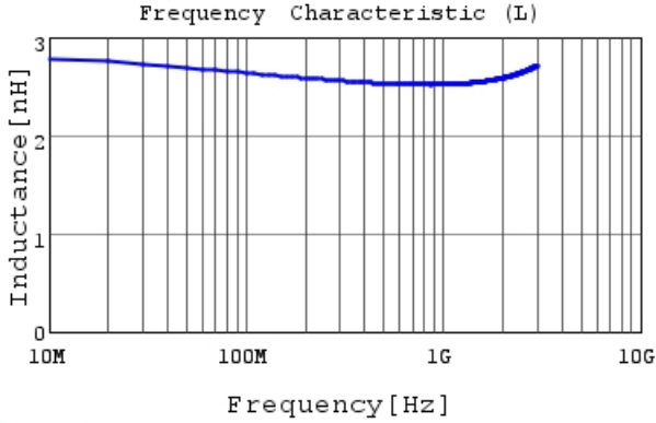
LQP03TN2N5B02 L
