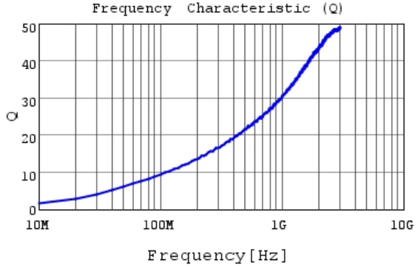
LQP03TN2N5B02 Q
