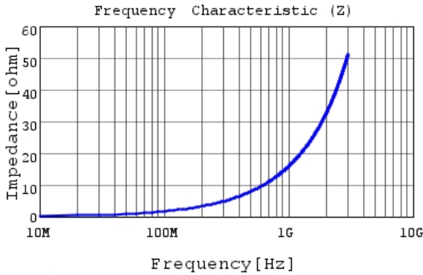
LQP03TN2N5B02 |Z|
