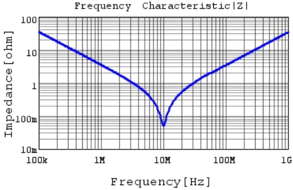
RDER72J473K3K1H03B |Z| DC0V, 25degC
