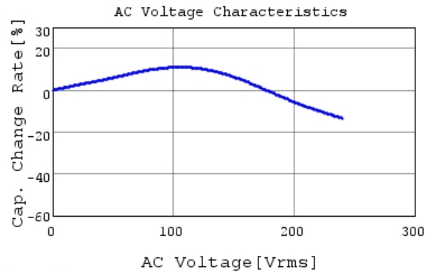
RDER72J473K3K1H03B C-AC Voltage capchange, I
