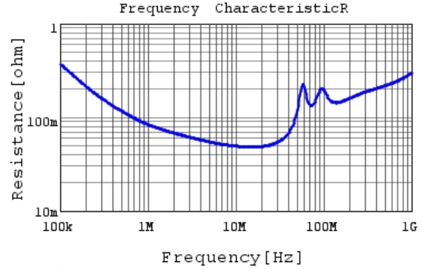
RDER72J473K3K1H03B R DC0V, 25degC
