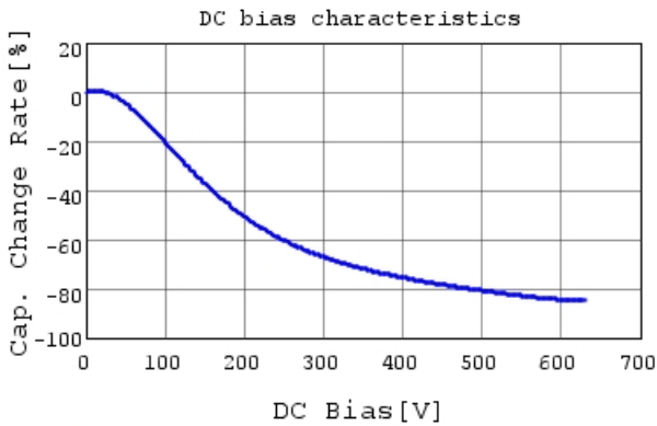
RDER72J473K3K1H03B C-DC bias capchange, 25.0
