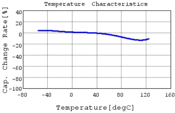
RDER72J473K3K1H03B C-Temp. capchange, DCOV,
