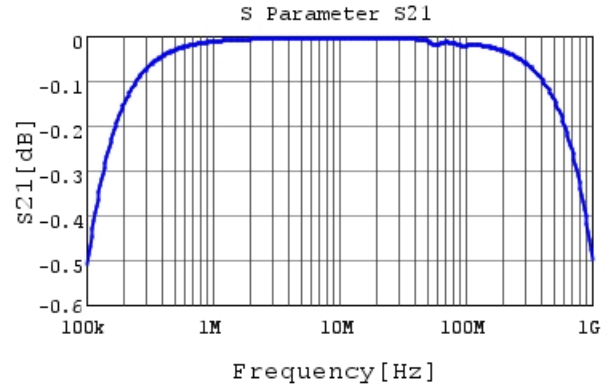
RDER72J473K3K1H03B S21 DCOV, 25degC
