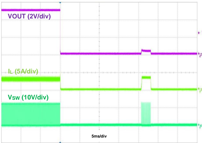
Figure 12. Output Short Protection, IOUT = 3A
