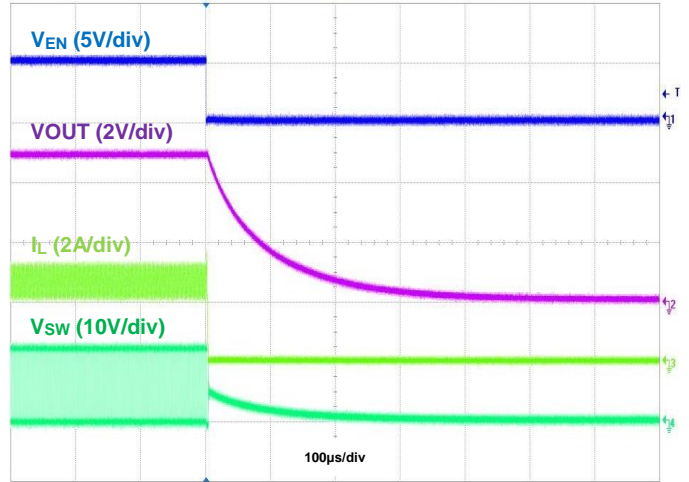
Figure 11. Shutdown Using EN, IOUT = 3A
