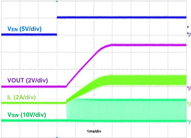
Figure 10. Startup Using EN, IOUT = 3A
