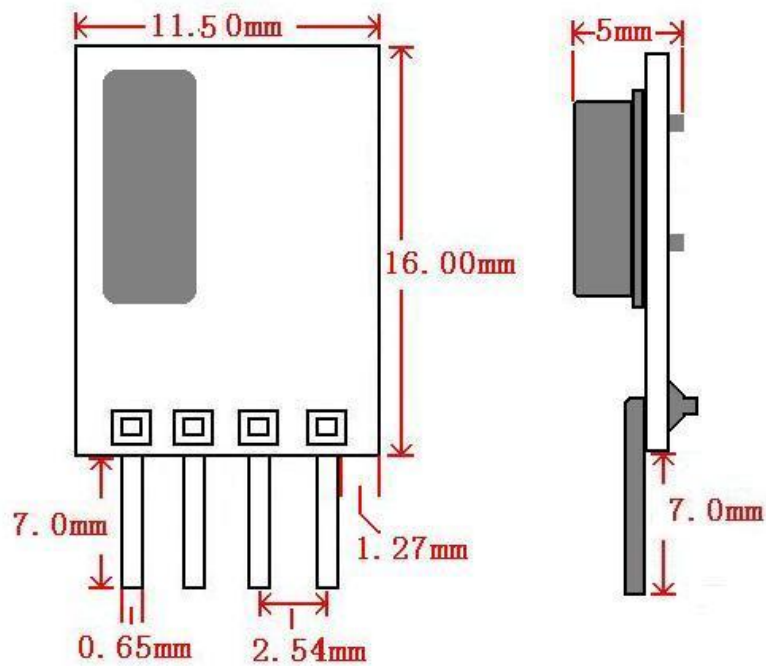
Figure1 CYT5 Dimension
